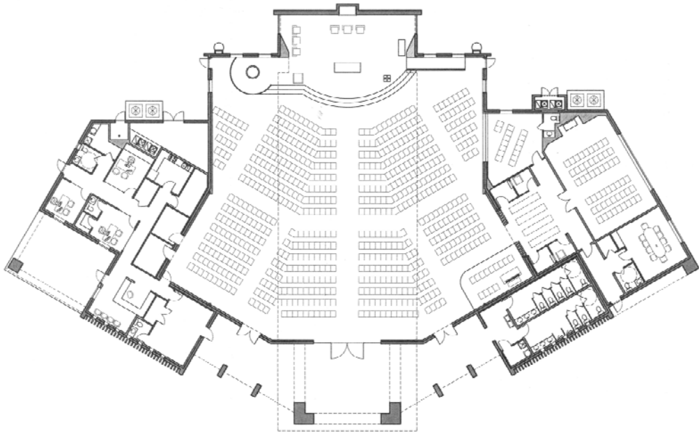
FLOOR PLAN
